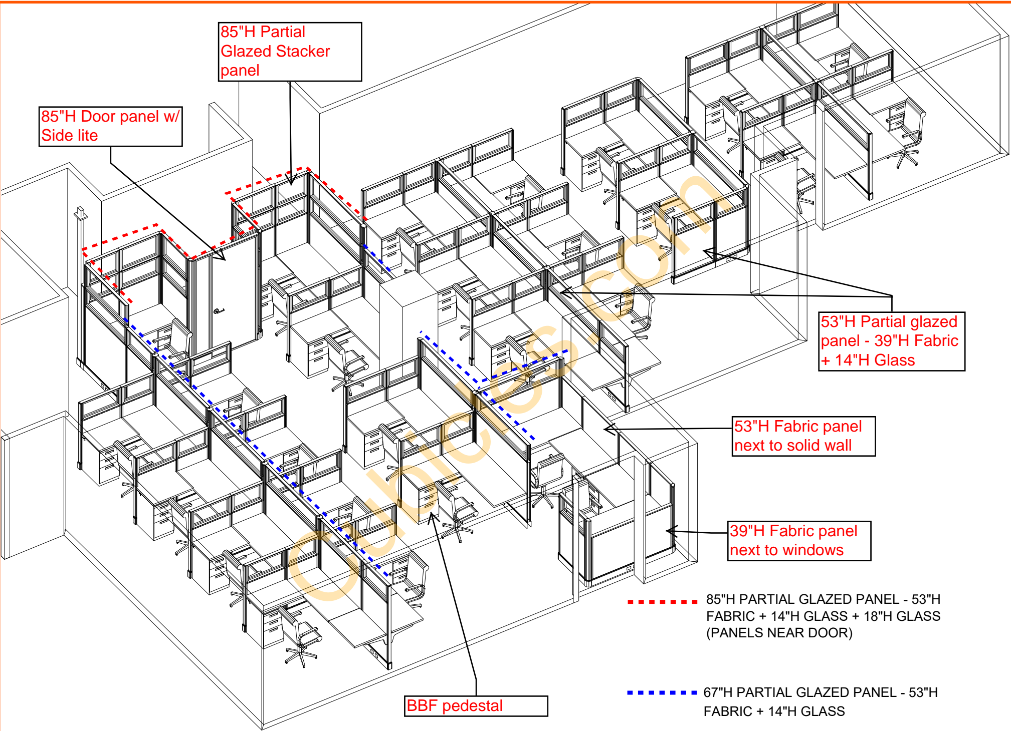
3D LAYOUT
