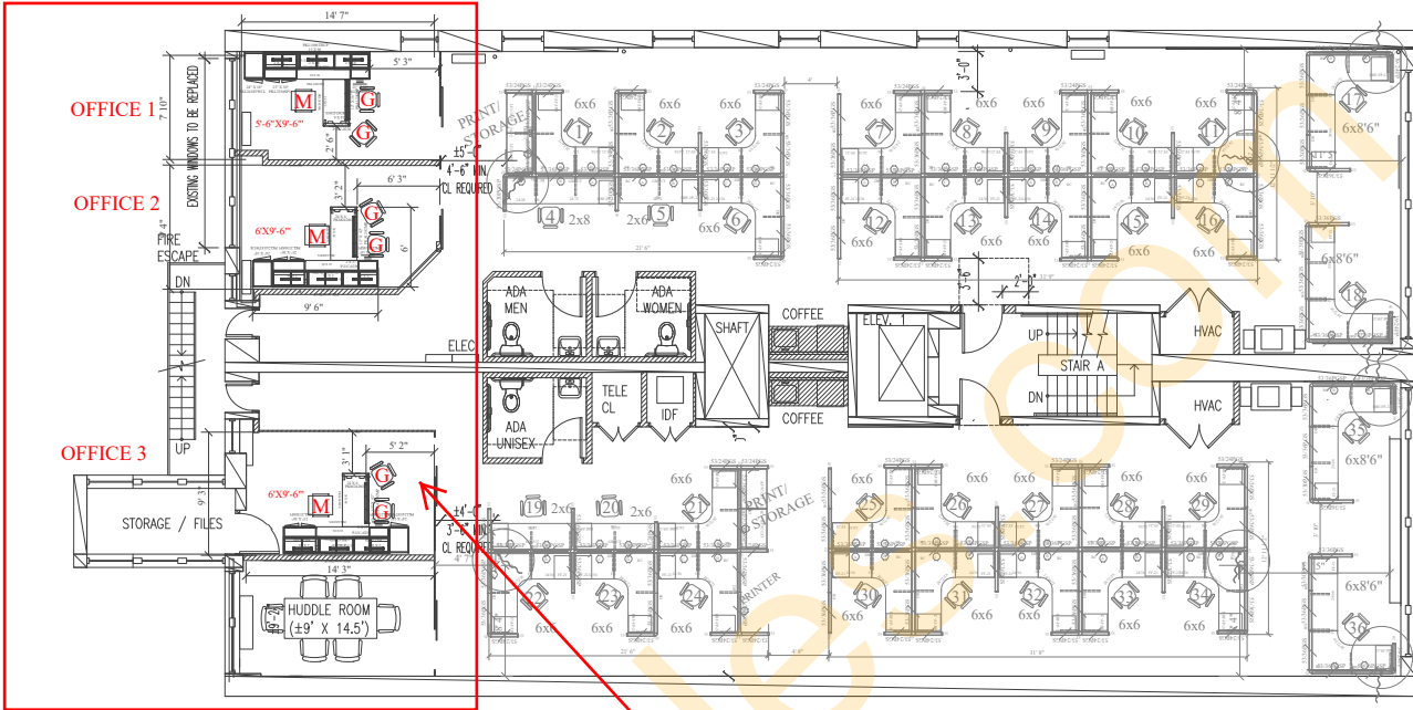
7th floor
