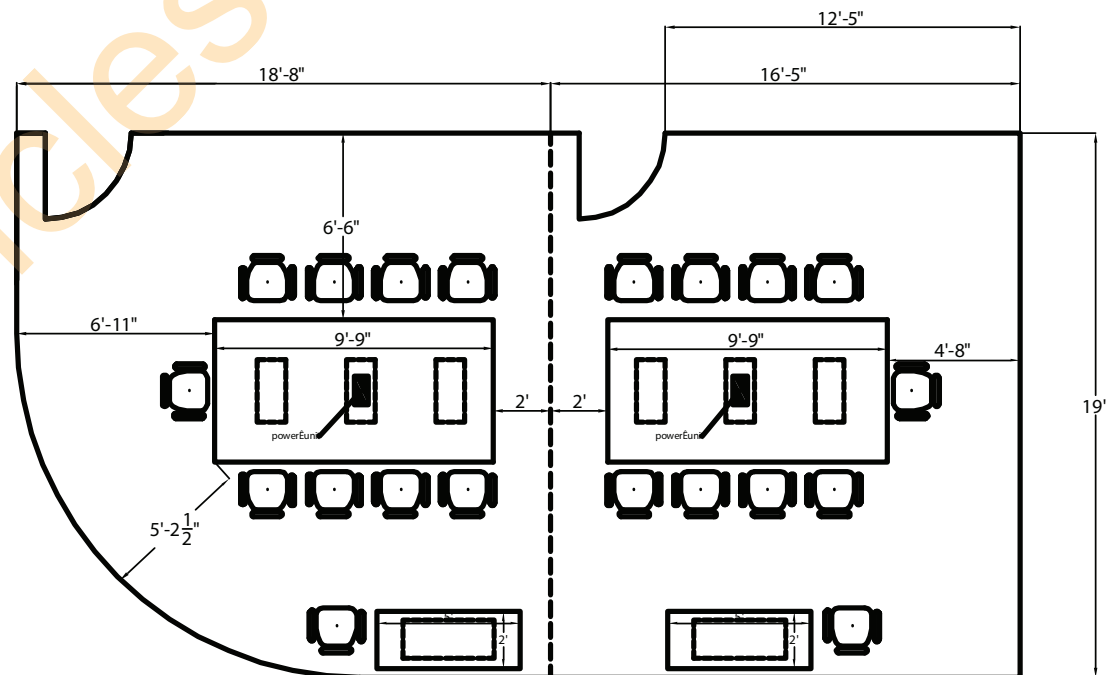
2D Layout - #314
